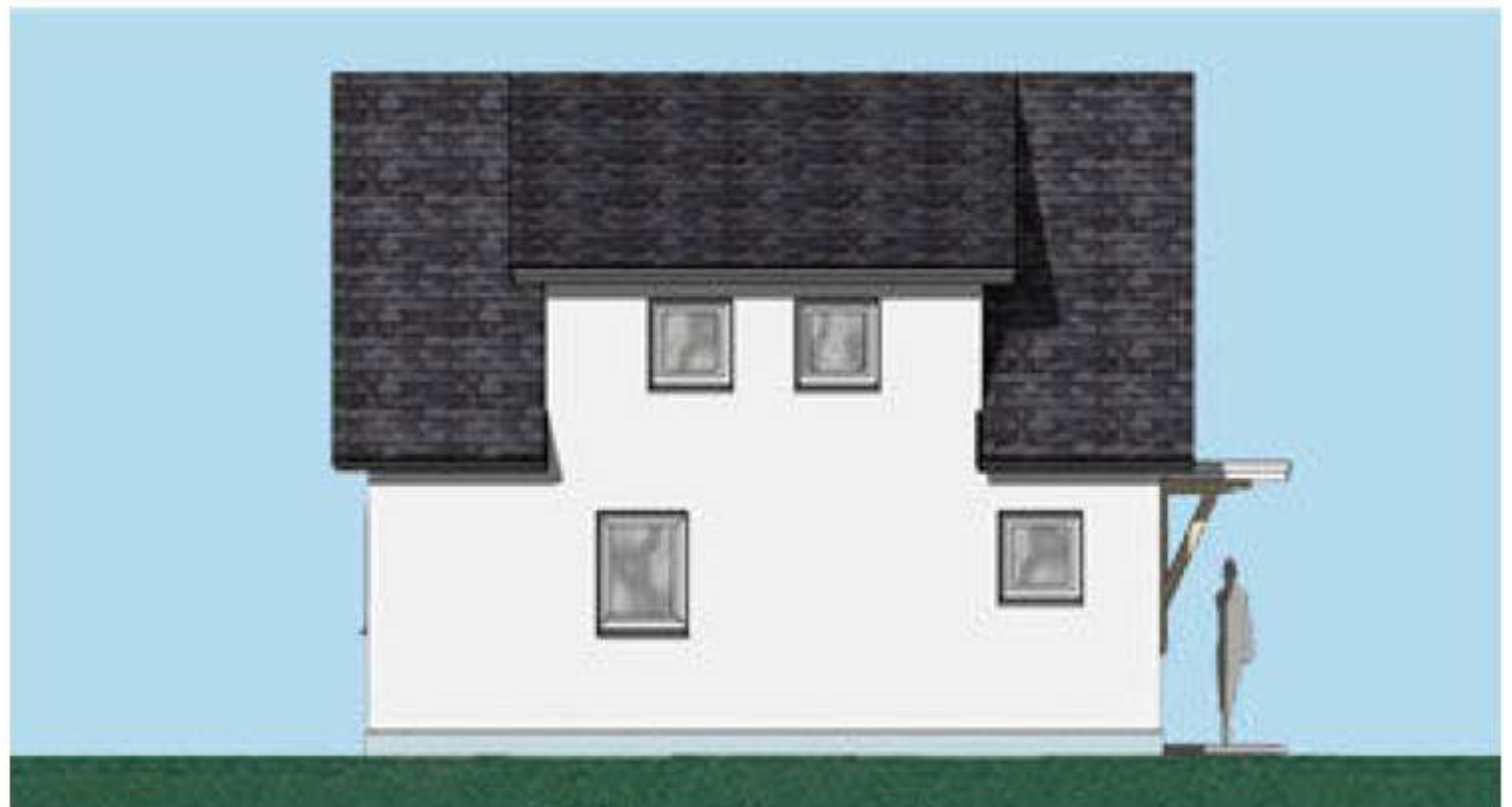
SIDE ELEVATION
