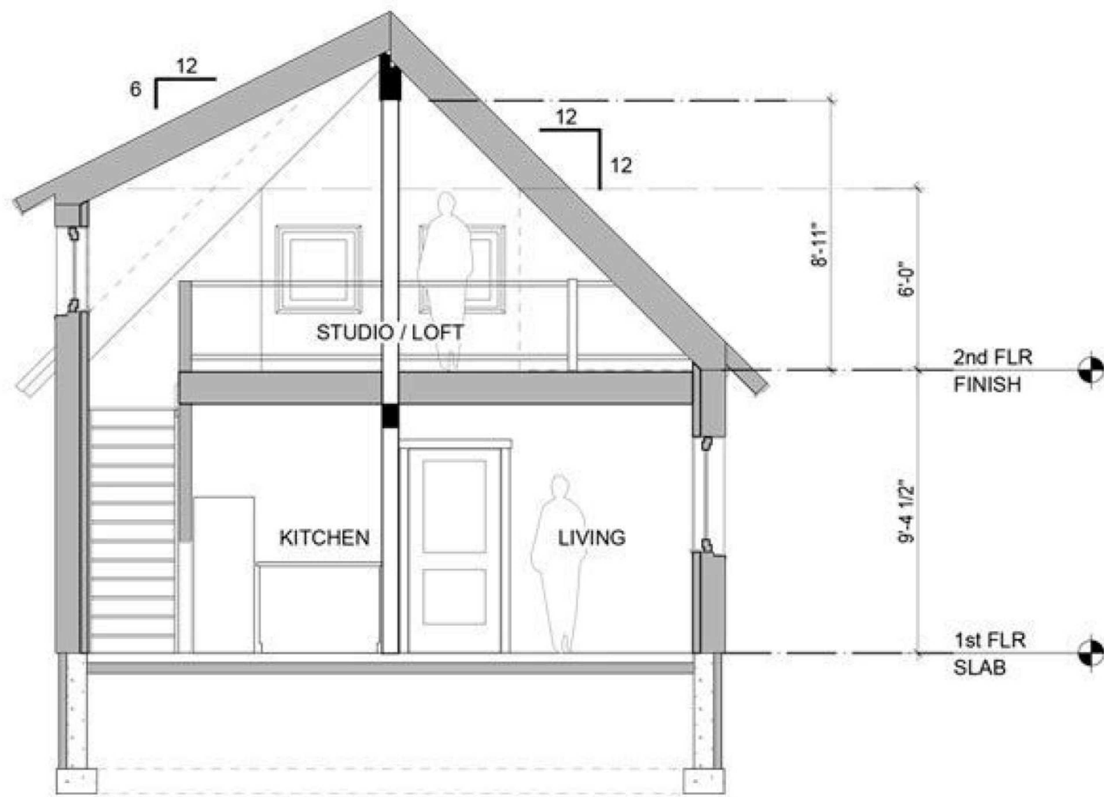
SECTION AT DORMER ROOF
