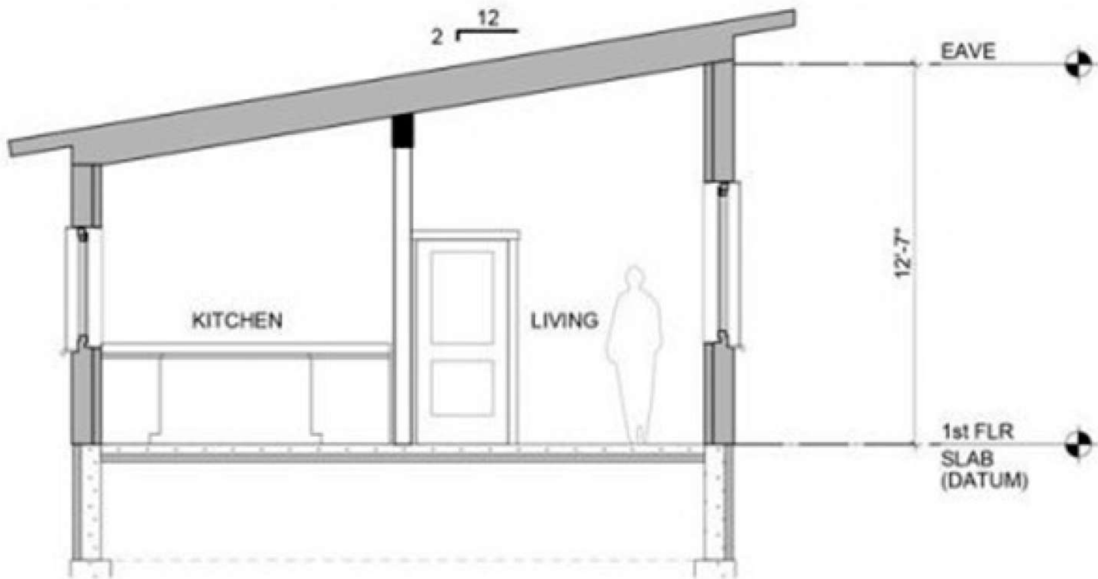
SECTION AT LIVING ROOM
