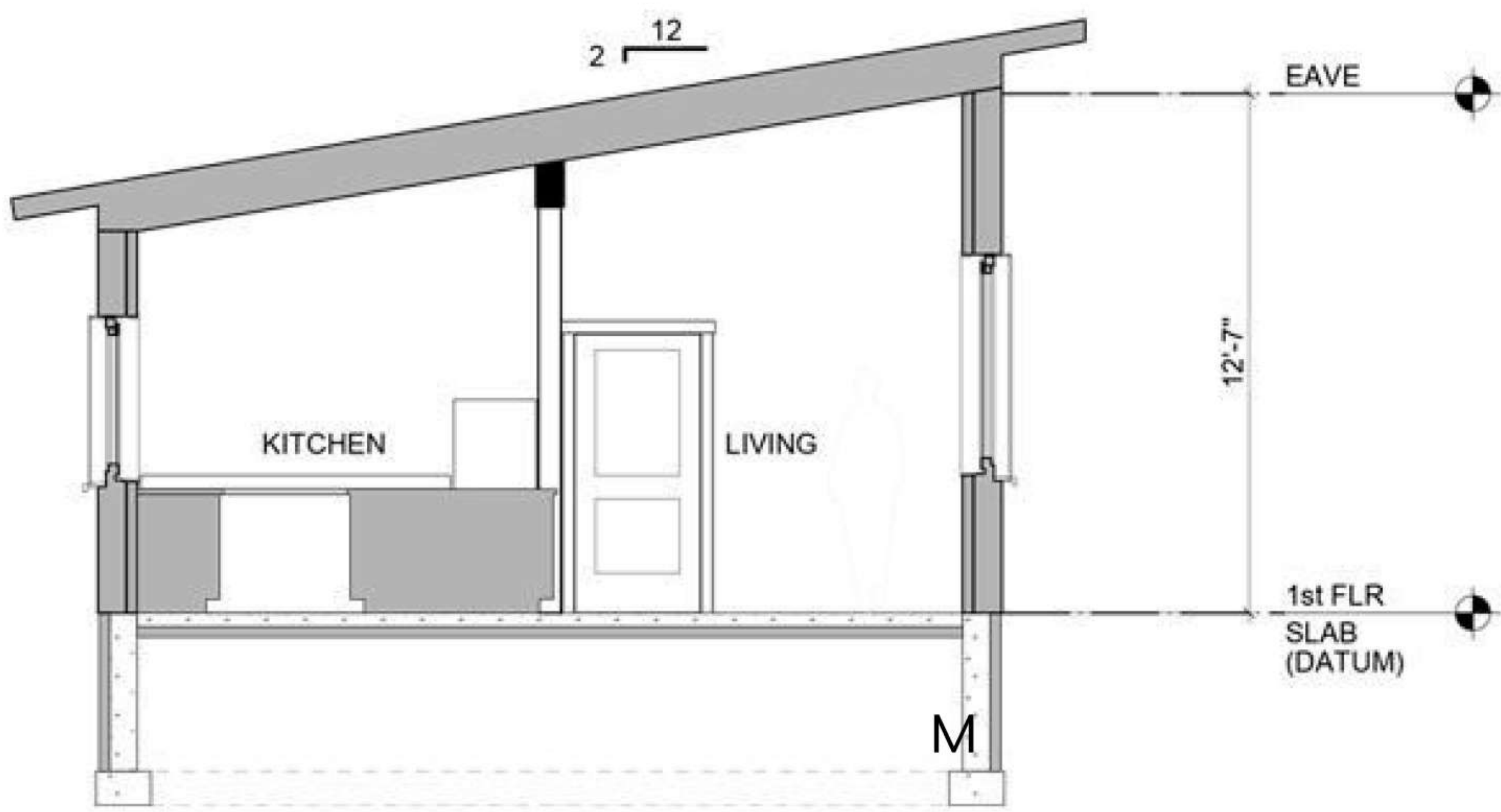
SECTION AT LIVING ROOM
